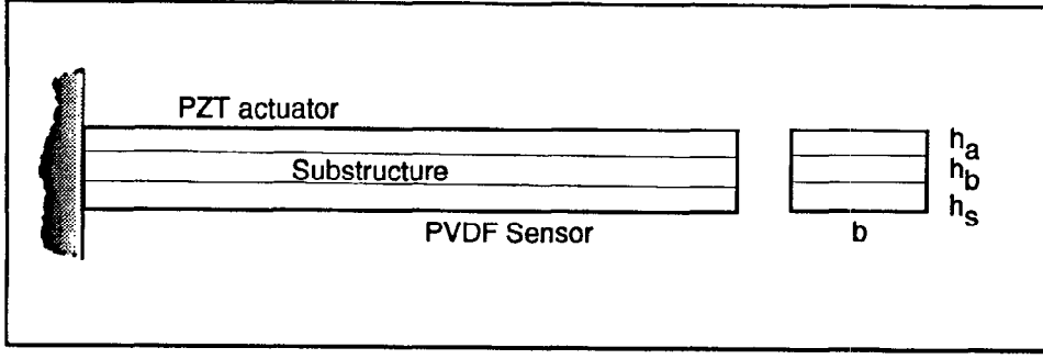
Figure 1: The composite beam
