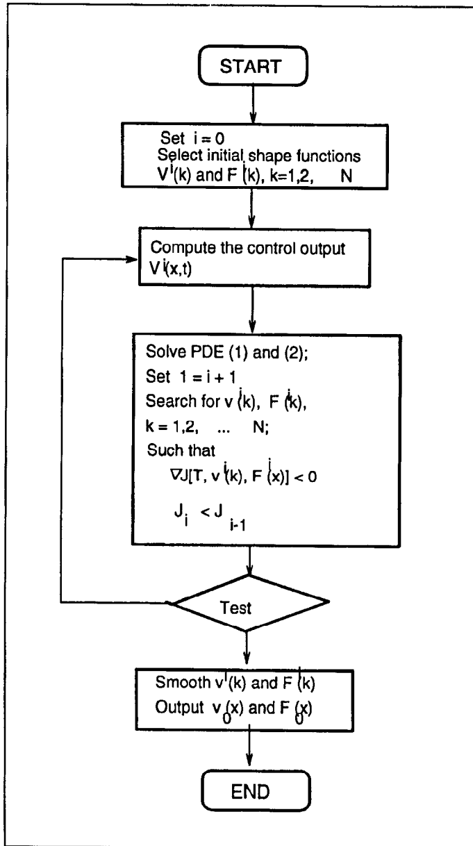
Figure 4: Optimization algorithm
