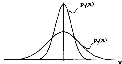
Figure 1: Plot of two pattern densities
