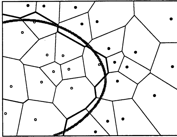
Figure 3: Voronoi vectors and their approximate decision region.
