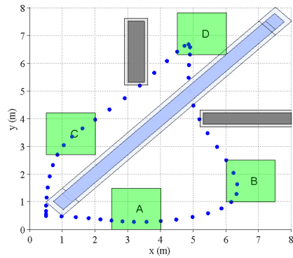
Fig. 5. Workspace setup of the second test case. The moving obstacle moves from the the bottom left corner to upper right corner. 2D trajectory of the vehicle is shown as blue dots. The resulting motion is clockwise.
