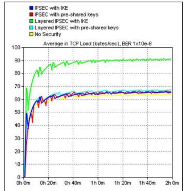
Fig. 5. Average TCP load at client for BER 1 \times 10^{-6} .
