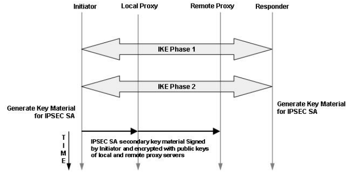
Fig. 2. Addition to IKE handshake mechanism for LES key management
