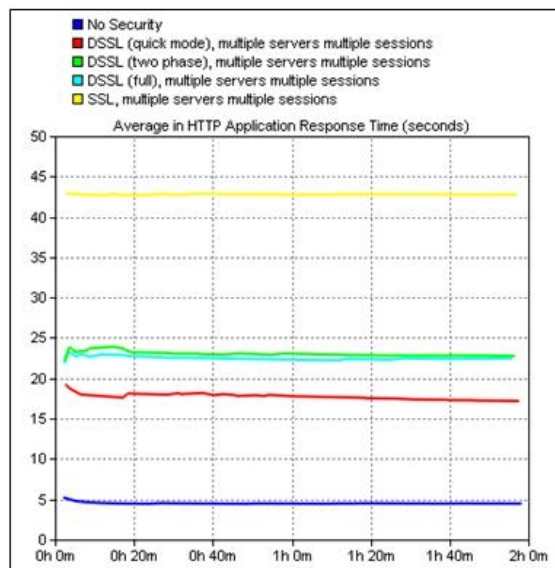
Fig. 8. HTTP response times for different versions of DSSL and comparison to SSL and unsecured web browsing.
