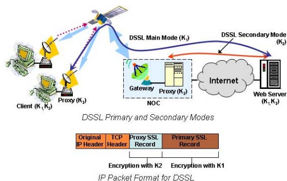
Fig. 3. Dual-Mode SSL for HTTP optimization
