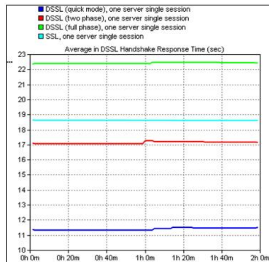
Fig. 7. Handshake time comparison for DSSL versions and SSL.
