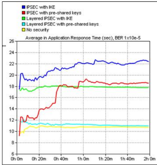
Fig. 4. Comparison of custom application response time (global average) for satellite link BER 1 \times 10^{-5} .
