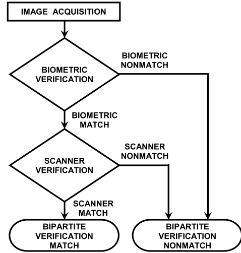
Fig. 14. Bipartite verification.
