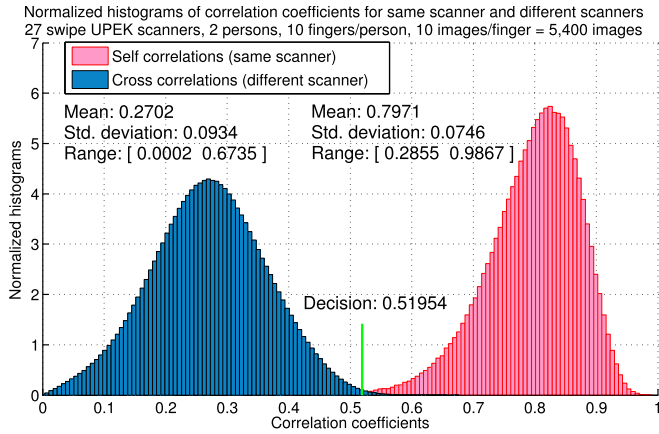
Fig. 12. Histograms of self correlations and cross correlations in inverse mode.
