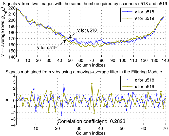
Fig. 10. Input and output signals of the moving-average filtering in direct mode.
