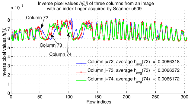
Fig. 5. Inverse pixel values h(i, j) of 3 adjacent columns and their averages.
