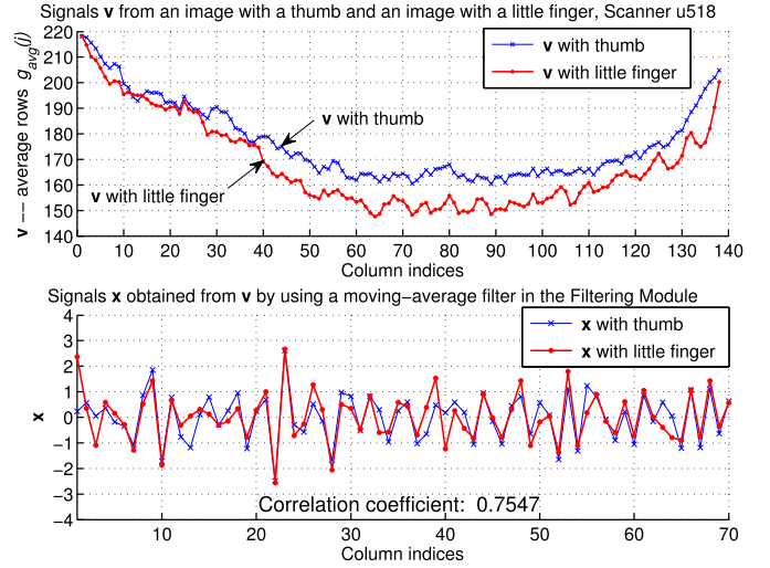
Fig. 8. Input and output signals of the moving-average filtering in direct mode.
