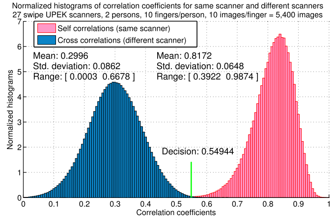
Fig. 11. Histograms of self correlations and cross correlations in direct mode.
