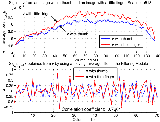
Fig. 9. Input and output signals of the moving-average filtering in inverse mode.
